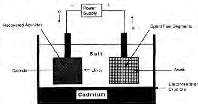
Fig. 1. Electrorefiner schematic.
