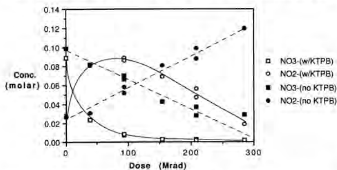
Fig. 4. Nitrate and Nitrite Changes during Co-60 Gamma Radiolysis of a Simulated Nuclear Waste Solution in the Absence and Presence of 10 wt% KTPB Precipitate. ---, KTPB Absent; ———, KTPB Present.
