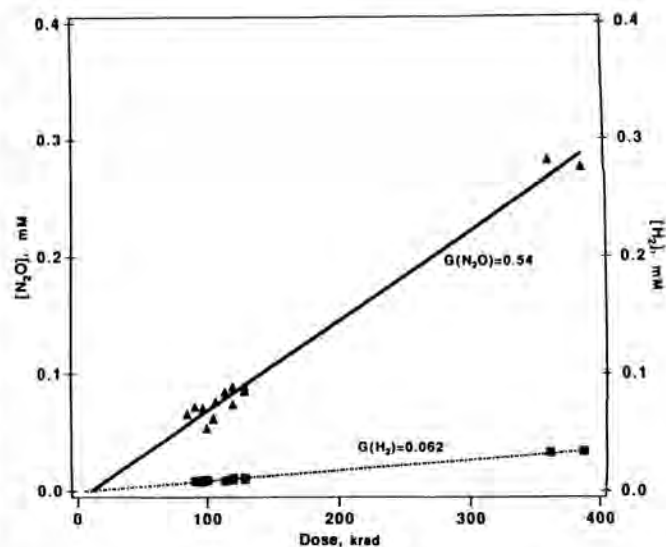
Fig. 2. Nitrous oxide and hydrogen production from Co-60 gamma radiolysis of a simulated nuclear waste solution containing organic. ( \text{NaOH} = 2.0 \text{ M} , \text{NaNO}_3 = 2.8 \text{ M} , \text{NaNO}_2 = 2.2 \text{ M} , \text{NaAlO}_2 = 1.3 \text{ M} and 0.085 M HEDTA and EDTA)
