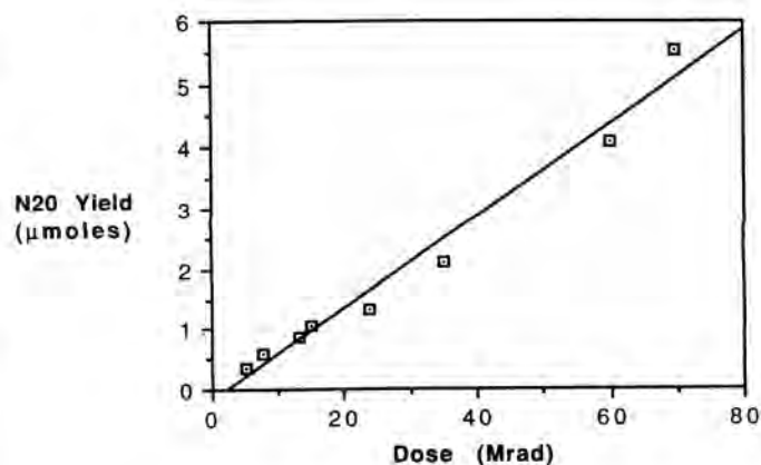
Fig. 3. Nitrous Oxide Gas yield from Co-60 Gamma Radiolysis of a 10 wt % Potassium Tetraphenylborate slurry containing 1.9 M NaNO 3 , 1.6 M NaOH, and 0.75 M NaNO 2 .
