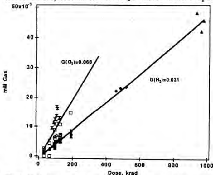
Fig. 1. Hydrogen and oxygen production from Co-60 gamma radiolysis of a simulated nuclear waste solution. ( \text{NaOH} = 2.0 \text{ M} , \text{NaNO}_3 = 2.8 \text{ M} , \text{NaNO}_2 = 2.2 \text{ M} , and \text{NaAlO}_2 = 1.3 \text{ M} ).
