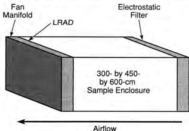
Fig. 8. Simplified drawing of large LRAD monitor system.
