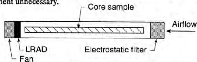
Fig. 10. Conceptual drawing of a core sample monitor.
