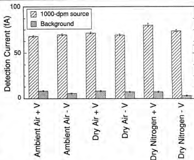
Fig. 5. Detector responses (source and background) of Fig. 4 analyzed and plotted as a function of source strength.
