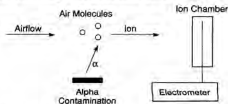
Fig. 2. Detection of air ions produced by alpha particles.
