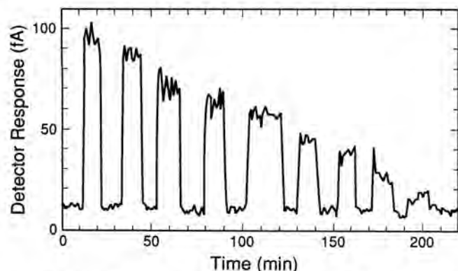
Fig. 4. LRAD response (from left to right) to ^{239}\text{Pu} sources, ranging from 1100 to 100 dpm. All 9 source strengths can be read from Fig. 5.
