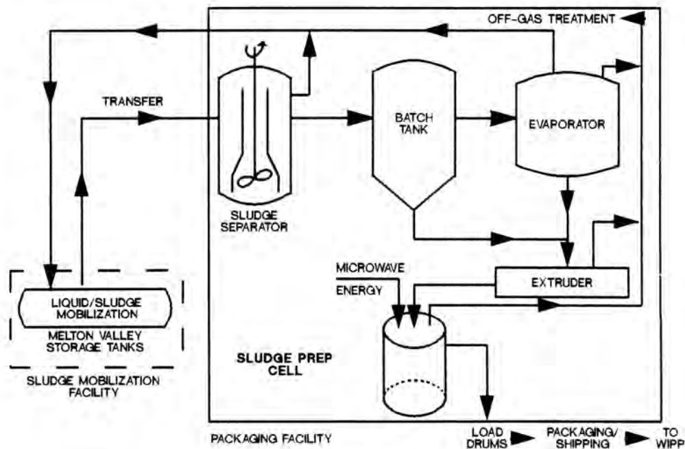
Fig. 2. WHPP Conceptual Slurry Processing Flow Sheet.
