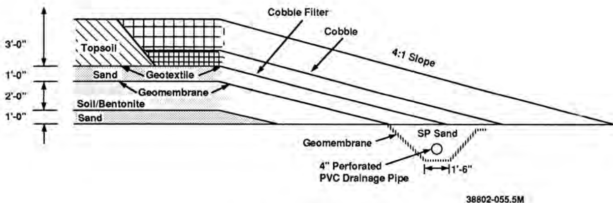
Fig. 5. Proposed Cover Details.
