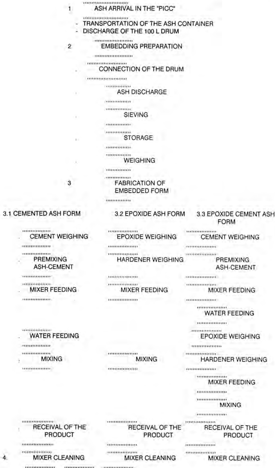
Fig. 4. The PICC Polyvalent Embedding Process Chart.
