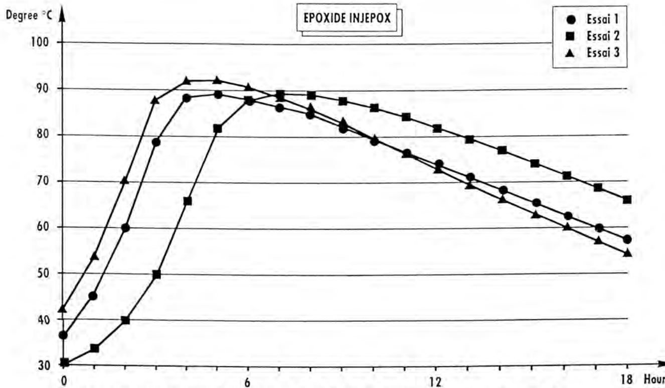
Fig. 8. Epoxide Cement Campaign-Polymerization Temperature-INJEPOX Epoxide.
