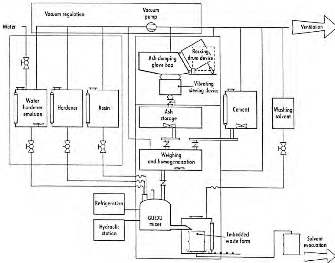
Fig. 2. PICC- Incinerator ash conditioning facility.
