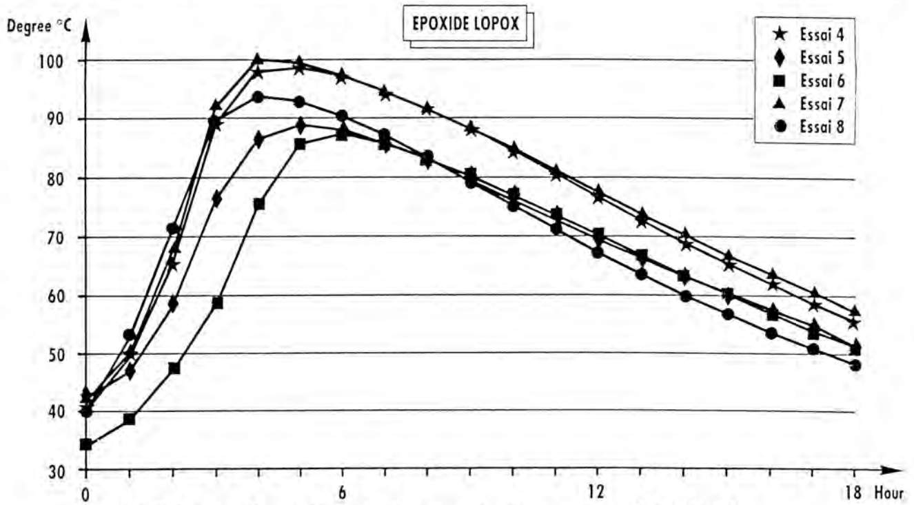
Fig. 7. Epoxide Cement Campaign-Polymerization Temperature LOPOX Epoxide.
