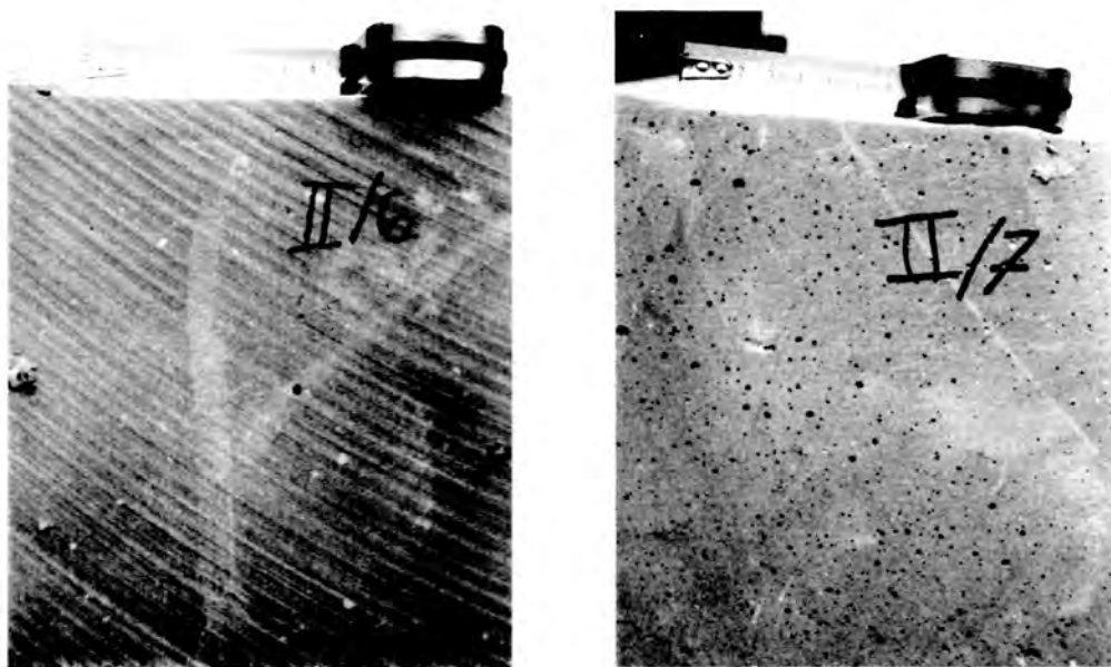
Fig. 5. Cemented Phosphated Ashes-Quality of the Product After Degassing.
