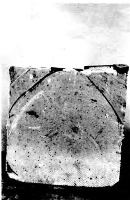
Fig. 6. Cemented Phosphated Ashes-Typical Crack.
