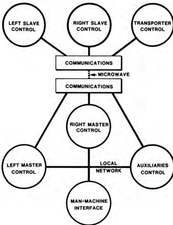
Fig. 6. Control system block diagram.
