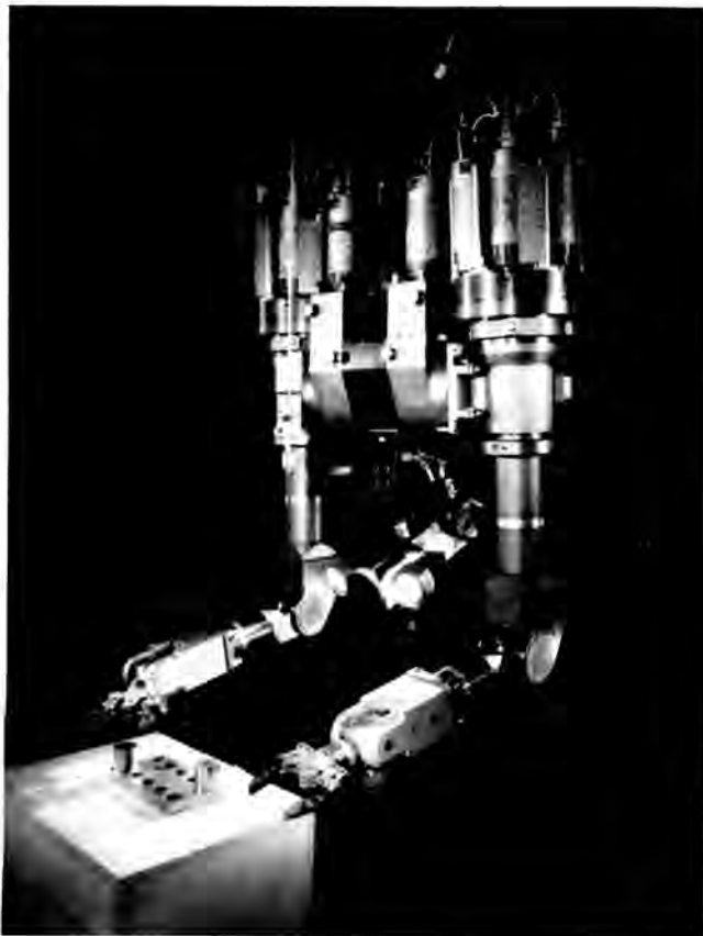
Fig. 2. Advanced servomanipulator slave arms.
