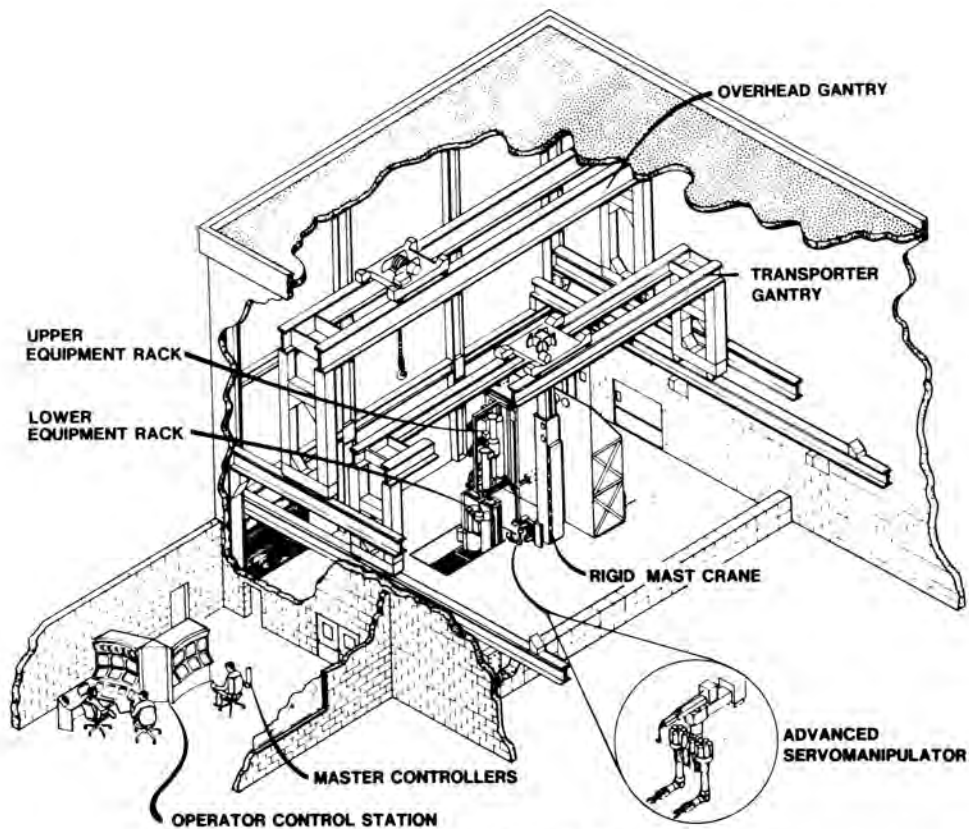
Fig. 1. Advanced Integrated Maintenance System.
