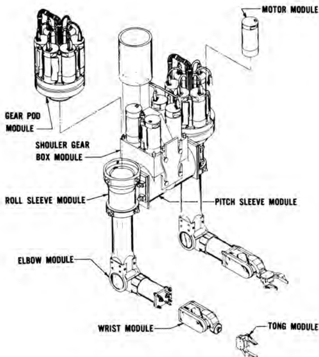
Fig. 3. Advanced servomanipulator slave arm modules.
