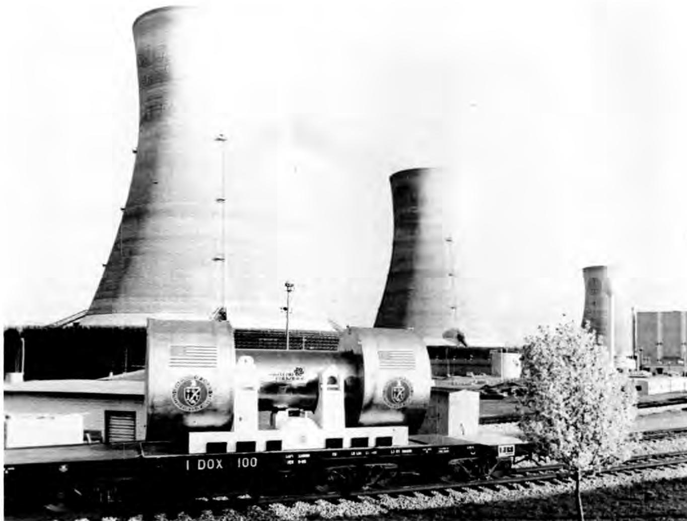
Fig. 1. NuPac 125-B Rail Cask at TMI. at TMI.
