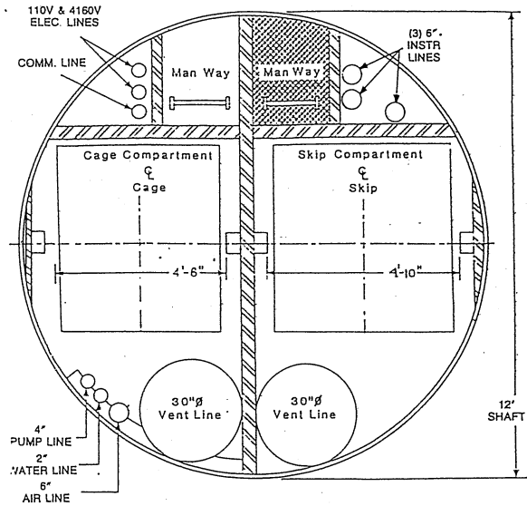
Figure 5. Shaft Section
