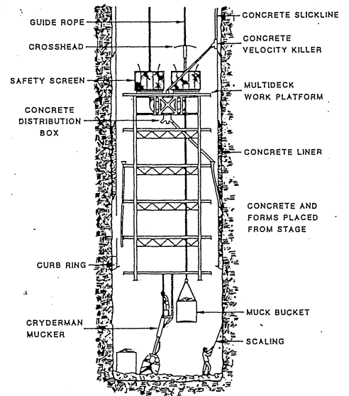
Figure 8. Shaft Sinking Process
