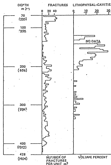
Figure 3. Fracture Frequency and Lithophysal Distribution (Ref. 1)
