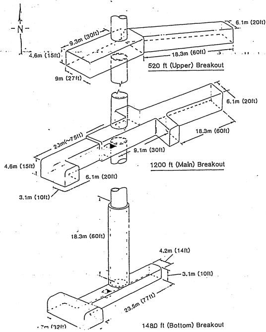
Figure 6. Lateral Subsurface Excavations
